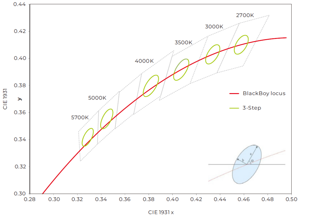
SDCM≤3 (3 step MacAdam ellipse)
